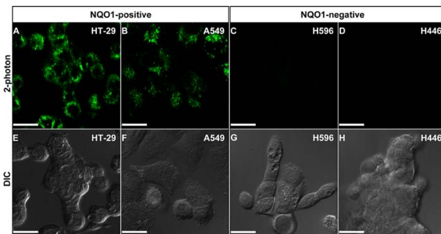
Figure 6. Two-photon confocal microscopy imaging of living HT-29 (A,E), A549 (B,F), H596 (C,G), and H446 (D,H) cells in the presence of 2.0 \times 10^{-5} M Q_3NI probe. Fluorescence images of each cell line are on the top row with their respective differential interference contrast (DIC) image on the bottom row. Images were acquired at \lambda_{ex} = 750 nm (3% laser power) without any washing steps between Q_3NI probe addition and imaging. Scale bars represent 2.5 \times 10^{-5} m.
