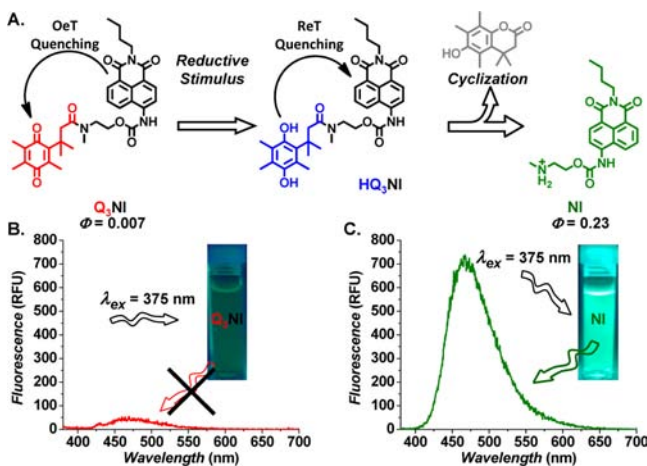
Figure 1. Schematic representation of the unique utilization of PeT quenching in the hNQO1 probe Q 3 NI and the emission properties associated with Q 3 NI probe and NI: (A) proposed quenching mechanisms for Q 3 NI probe prior to and after chemical/hNQO1-catalyzed reduction and subsequent production of the fluorescent NI reporter. Fluorescence spectra and optical images of cuvettes containing 2.0 \times 10^{-6} M solutions of (B) Q 3 NI probe and (C) NI reporter in pH 7.4, 0.1 M PBS that result from excitation at \lambda_{\text{ex}} = 375 nm (spectra) and \lambda_{\text{ex}} = 365 nm (images).
