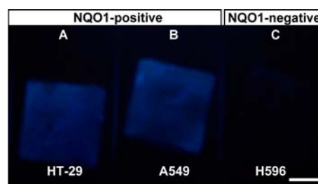
Figure 4. Visual differentiation of (A) HT-29, (B) A549, and (C) H596 cancer cells cultured on 2.2 \times 2.2 cm glass substrates after 10 min incubation with 2 \times 10^{-5} M Q_3NI probe. Images of cells were captured with a digital camera upon irradiation at \lambda_{ex} = 365 nm with a hand-held lamp. Scale bar represents 1 cm.
