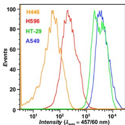
Figure 5. Flow cytometry assays of Q_3NI activation by hNQO1-positive (A549 and HT-29) and hNQO1-negative (H596 and H446) cancer cells. Assays were performed by counting 10 000 cells that had been exposed to 2.0 \times 10^{-5} M Q_3NI probe for 10 min; \lambda_{ex} = 405 nm, \lambda_{em} = 457/60 nm.
