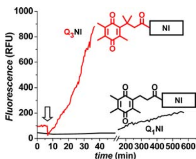
Figure 2. Comparing the dithionite-initiated formation of NI reporter from Q_3NI probe and Q_1NI . The fluorescence ( \lambda_{ex} = 370 nm, \lambda_{em} = 470 nm) from 3 mL solutions of 1.0 \times 10^{-5} M Q_3NI probe and Q_1NI in pH 7.4, 0.1 M PBS was monitored after their reduction by addition of 2.75 mg sodium dithionite (denoted by arrow).
