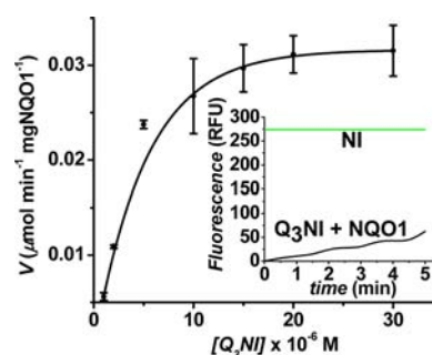
Figure 3. Kinetics plot of hNQO1 ( 2.0 \times 10^{-5} g) toward Q_3NI probe. Inset is an example of an assay observing fluorescent NI production from 1 \times 10^{-6} M Q_3NI , relative to signal for complete NI formation ( 1 \times 10^{-6} M). Values ( n = 3 ) are the average \pm 1 standard deviation.
